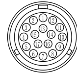
Feedback Connector Pinout
