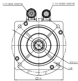
Mechanical View 3
