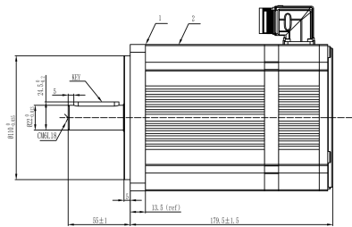
Mechanical View 4
