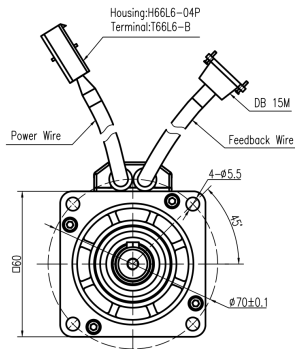
Mechanical View 1
