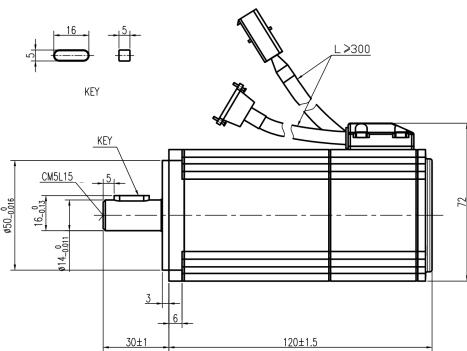
Mechanical View 3
