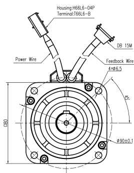
Mechanical View 1
