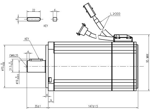
Mechanical View 3
