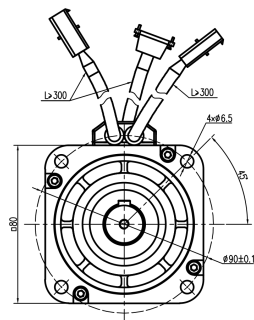
Mechanical View 3
