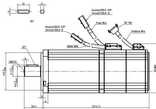
Mechanical View 1
