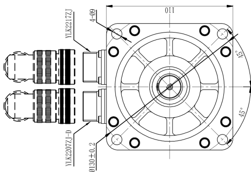
Mechanical View 1
