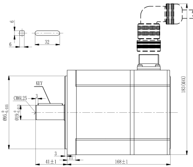
Mechanical View 3
