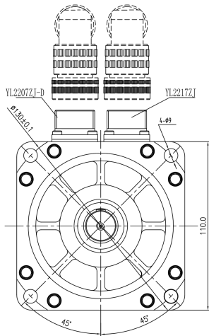
Mechanical View 1
