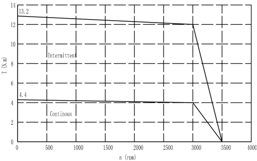
Torque-Speed Curve
