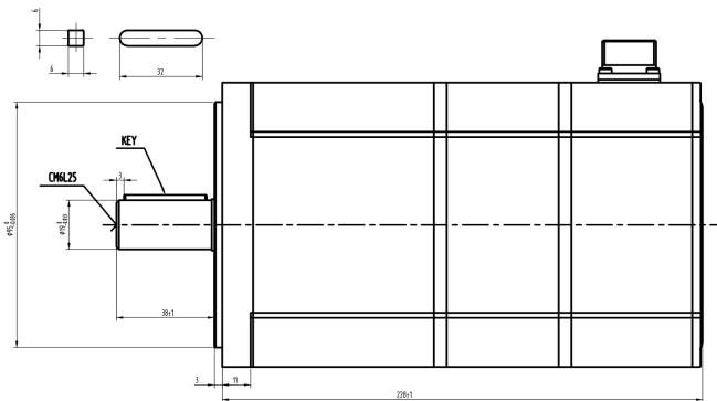
Mechanical View 1
