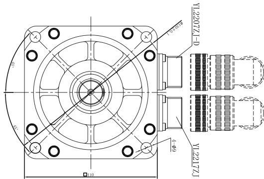
Mechanical View 1
