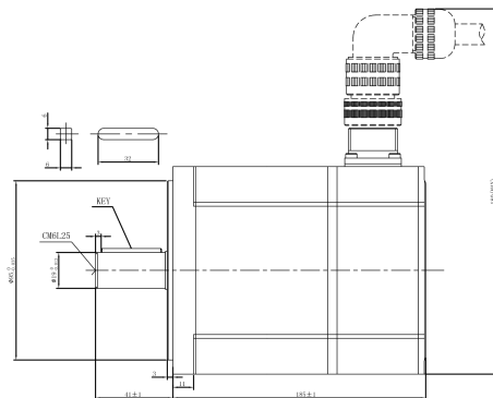
Mechanical View 3
