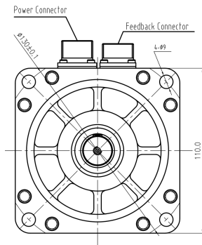
Mechanical View 1
