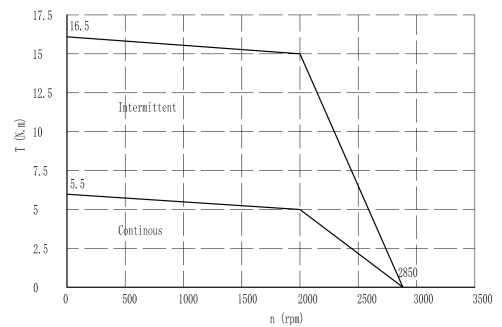
Torque-Speed Curve
