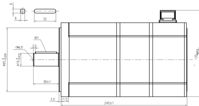
Mechanical View 3
