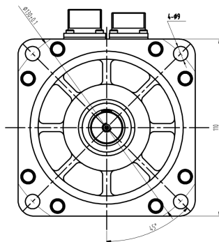
Mechanical View 3
