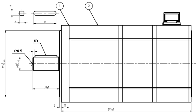
Mechanical View 1
