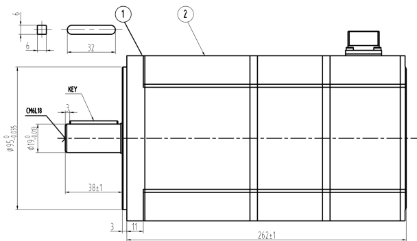
Mechanical View 3
