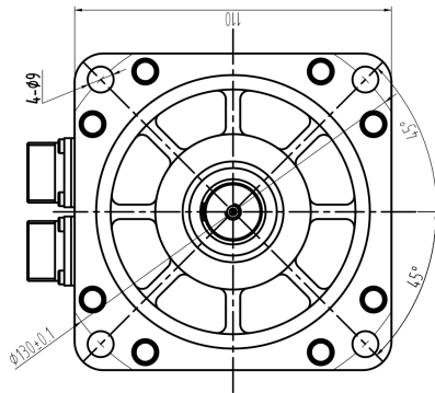
Mechanical View 1
