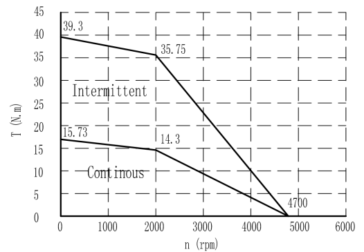
Torque-Speed Curve
