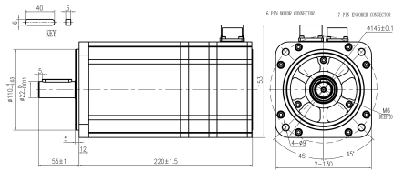
Mechanical View 1
