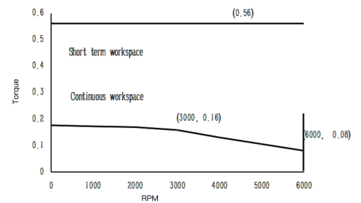
Torque-Speed Curve
