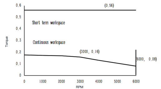
Torque-Speed Curve
