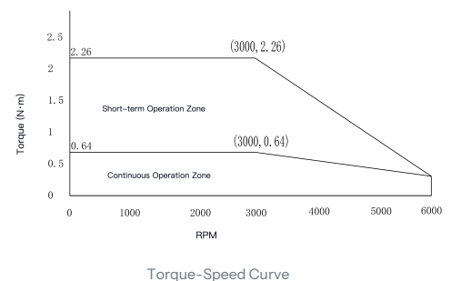
Torque-Speed Curve
