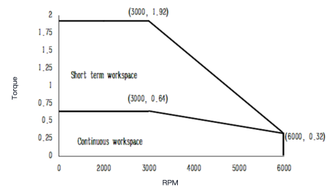
Torque-Speed Curve
