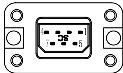
Feedback Connector Pinout
