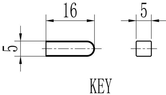
Mechanical View 1
