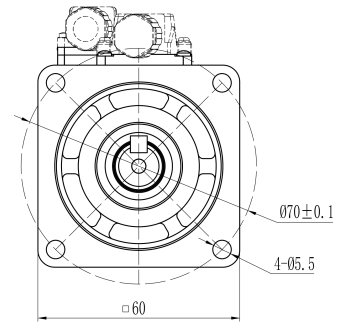
Mechanical View 2
