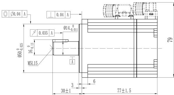
Mechanical View 3
