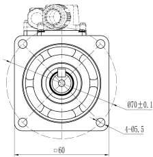
Mechanical View 3
