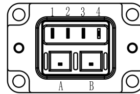
Power Connector Pinout
