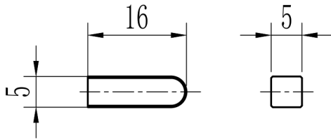
Mechanical View 1
