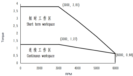
Torque-Speed Curve
