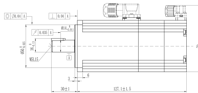
Mechanical View 4
