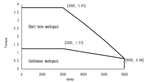
Torque-Speed Curve
