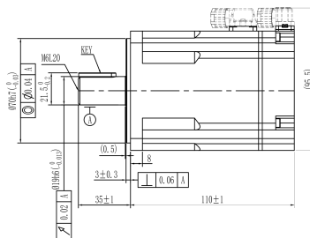
Mechanical View 4
