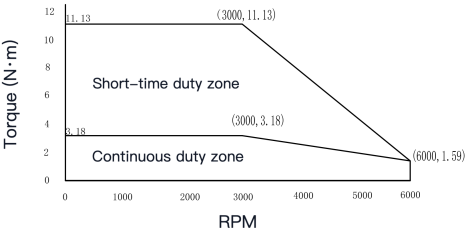
Torque-Speed Curve
