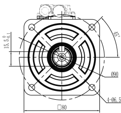
Mechanical View 3
