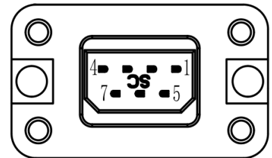
Feedback Connector Pinout
