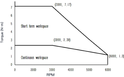
Torque-Speed Curve
