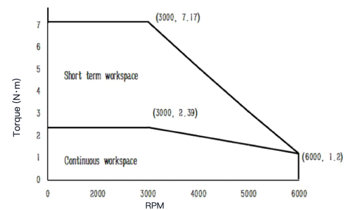
Torque-Speed Curve
