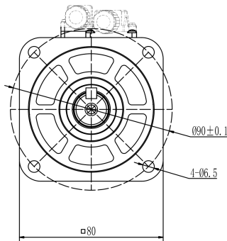
Mechanical View 3
