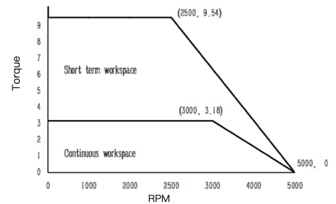
Torque-Speed Curve
