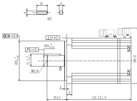
Mechanical View 1
