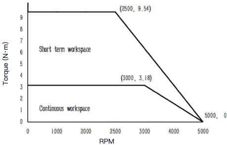
Torque-Speed Curve
