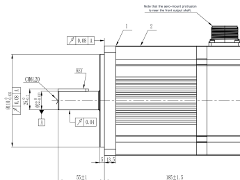
Mechanical View 4
