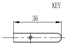
Mechanical View 1
