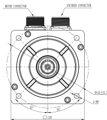
Mechanical View 3
