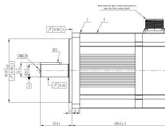
Mechanical View 4
