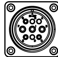
Power Connector Pinout
