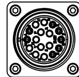
Feedback Connector Pinout
