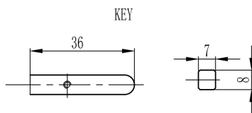
Mechanical View 1
