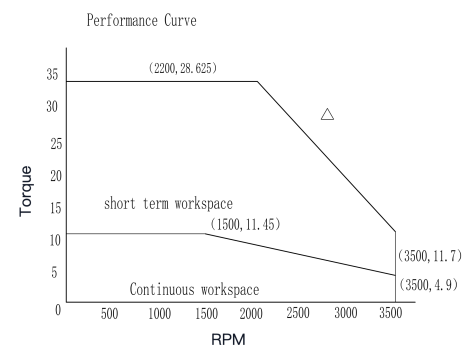
Torque-Speed Curve
