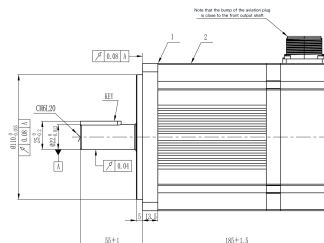
Mechanical View 4
