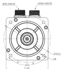
Mechanical View 3
