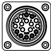
Power Connector Pinout
