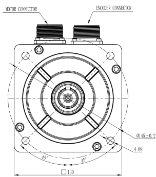
Mechanical View 3
