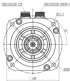
Mechanical View 1
