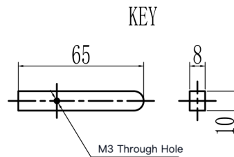
Mechanical View 4
