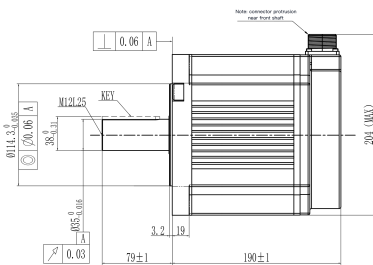
Mechanical View 3
