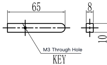
Mechanical View 4
