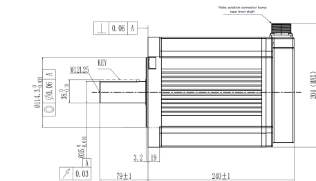
Mechanical View 1
