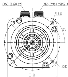
Mechanical View 3
