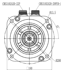
Mechanical View 1
