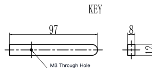
Mechanical View 4
