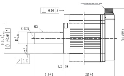
Mechanical View 3
