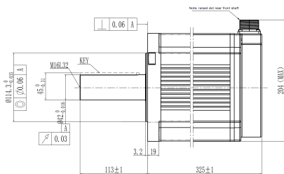
Mechanical View 3
