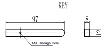
Mechanical View 4
