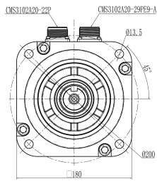
Mechanical View 1
