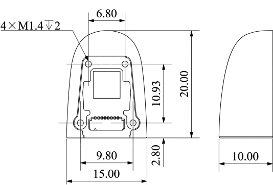
Mechanical View 1
