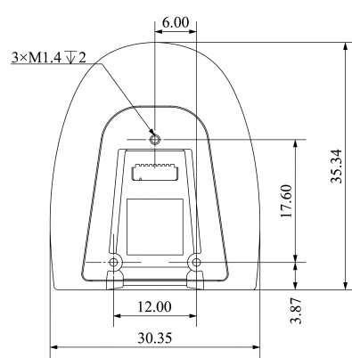
Mechanical View 1
