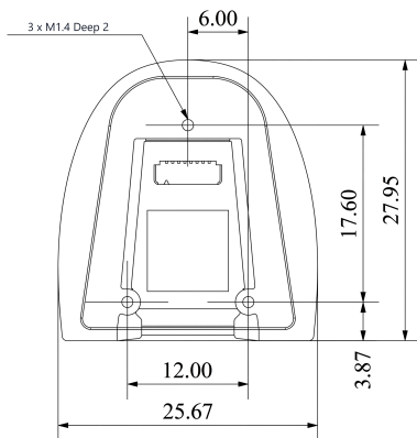
Mechanical View 1
