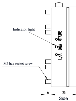
Mechanical View 3
