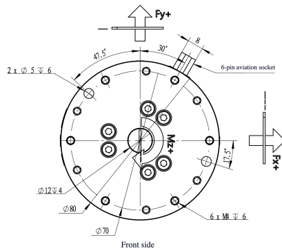
Mechanical View 1
