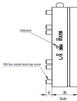
Mechanical View 3
