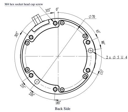
Mechanical View 2
