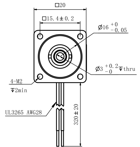
Mechanical View 3
