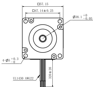
Mechanical View 1
