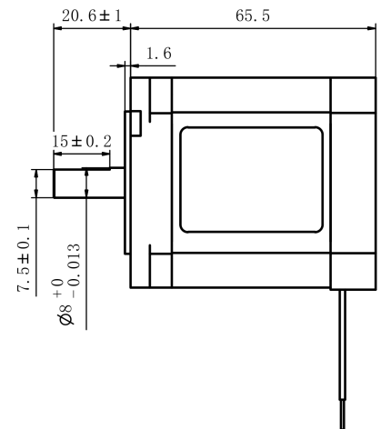
Mechanical View 3
