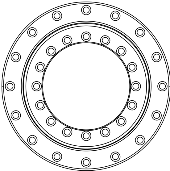
Mechanical View 3
