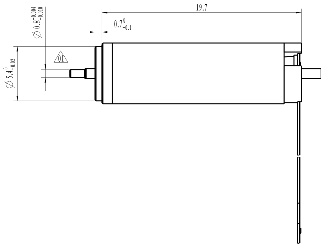
Mechanical View 1
