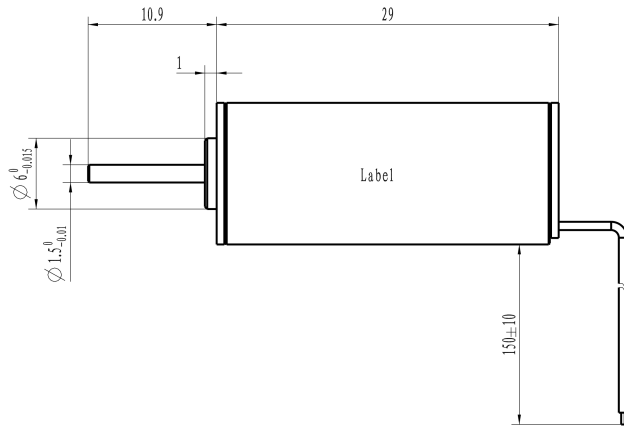
Mechanical View 1
