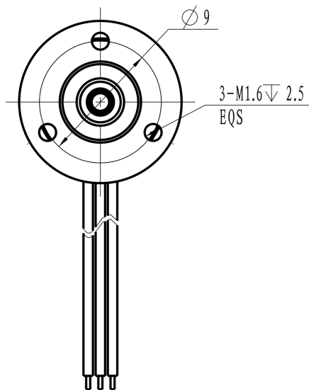
Mechanical View 3
