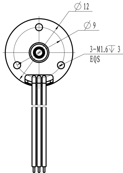
Mechanical View 2
