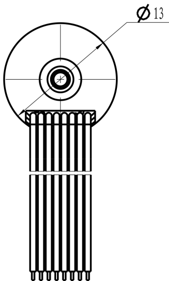
Mechanical View 3
