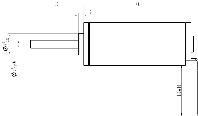
Mechanical View 1
