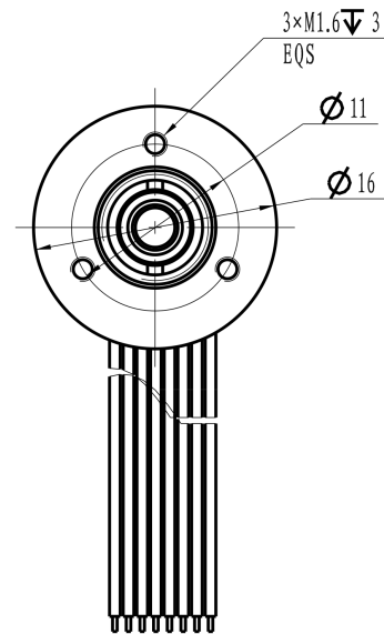
Mechanical View 2
