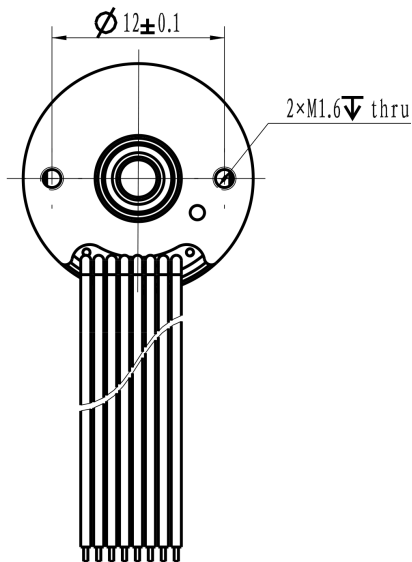
Mechanical View 3
