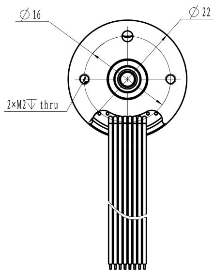
Mechanical View 3
