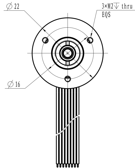
Mechanical View 2
