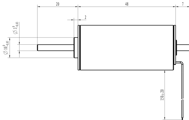
Mechanical View 1
