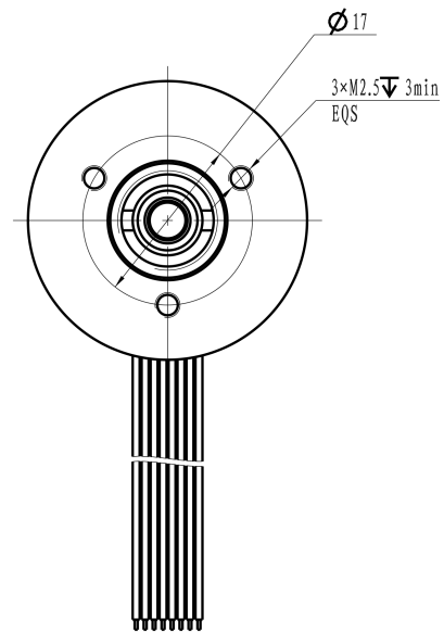
Mechanical View 2
