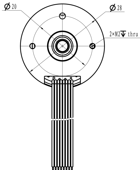
Mechanical View 3
