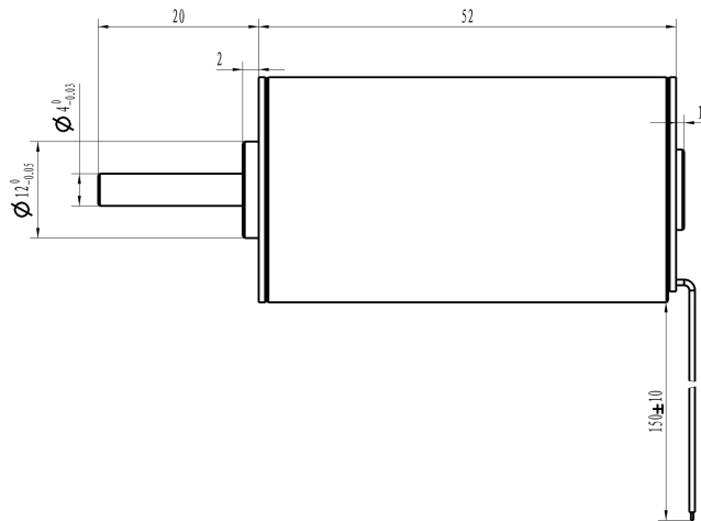
Mechanical View 1
