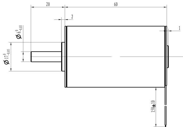
Mechanical View 1
