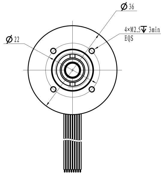
Mechanical View 2
