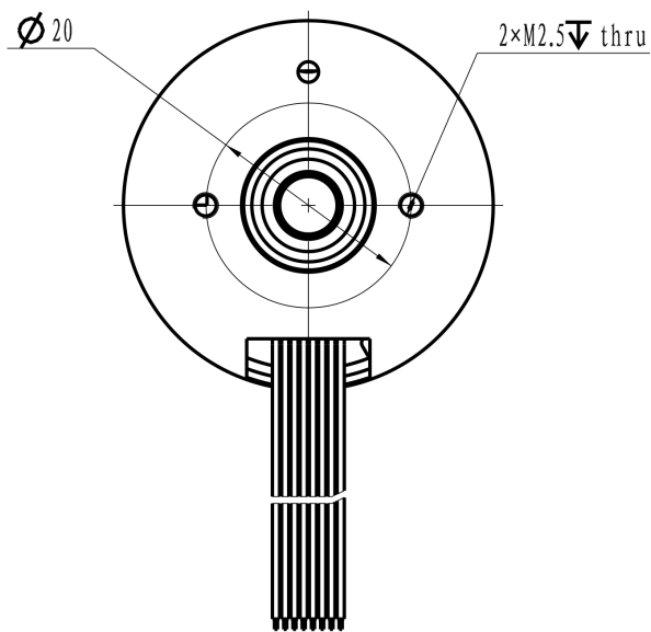
Mechanical View 3
