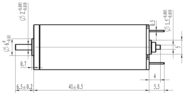
Mechanical View 1
