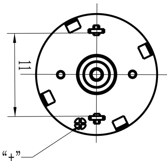
Mechanical View 3
