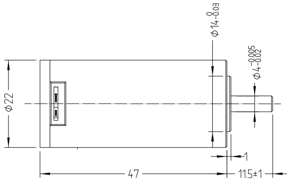
Mechanical View 1
