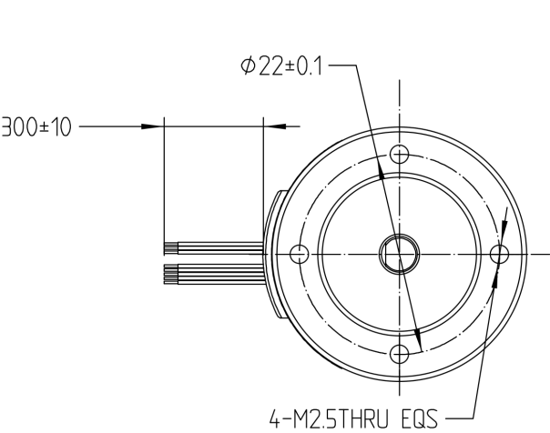
Mechanical View 1
