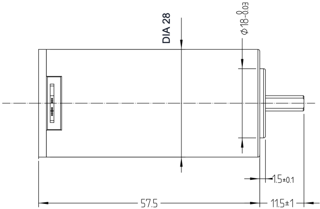
Mechanical View 2
